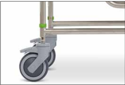
Telescopic castor tubes provide up to 100mm of height adjustment
